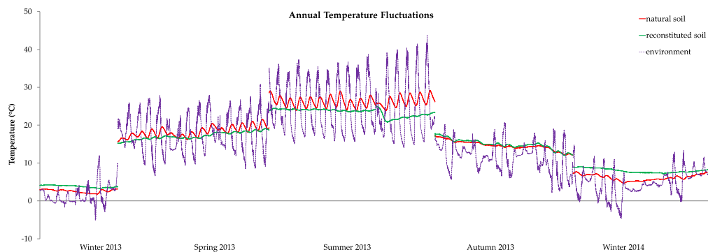
Fig. 10. Area 1, soil temperature fluctuations.
