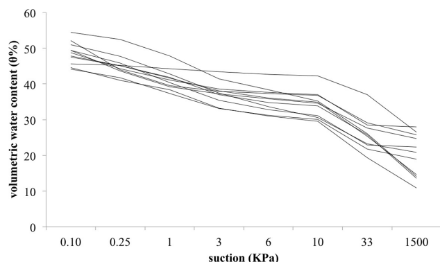
Figure 1. Water retention curves of sampled soils.
