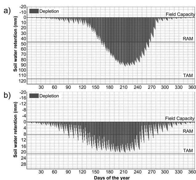
Figure 11. Water lost from agricultural soil (a) and from the landfill cover soil (b) by Crop Wat 8.0 software. Legend: RAM represents readily available moisture; TAM represents total available moisture.
