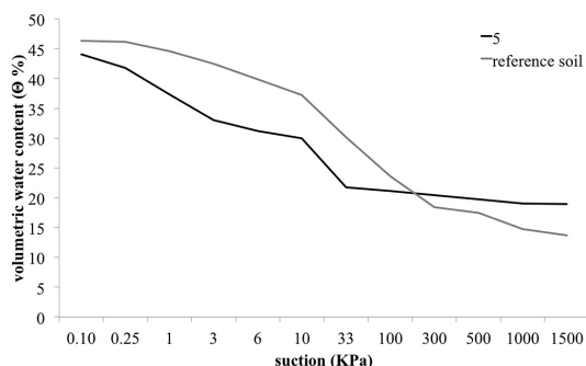
Figure 4. Comparison between sample 5 water retention curve and the reference curve – described as the arithmetic mean of PTFs values.
