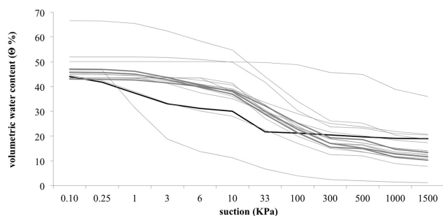
Figure 2. Sample 5: actual (black) and PTF water retention curves; the curves by Wösten et al. 1999 are highlighted.
