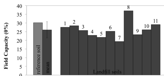
Figure 6. Volumetric water content ( \theta %) at field capacity: comparison between reference soil and landfill soils.
