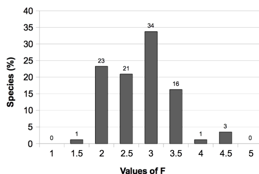
Figure 10. F index (soil moisture). Percentages are weighted by the frequency of the species in the monitoring sites (see column “Presence” in the Appendix). Legend: 1 is very dry, 1.5 is dry, 2 is moderately dry, 2.5 is fresh, 3 is moderately moist, 3.5 is moist, 4 is very moist, 4.5 is wet and 5 is flooded or submerged.
